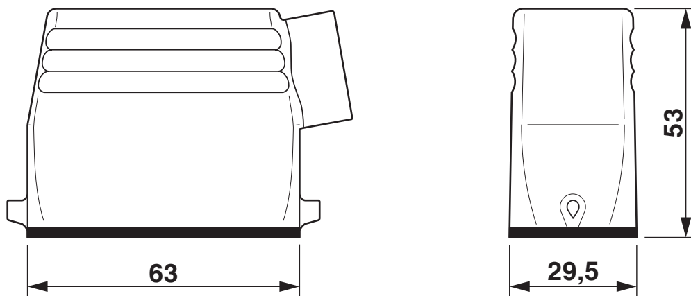
Dimensional drawing
